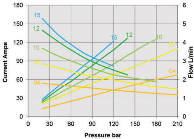
3" 12v 500w motor-pump performance
